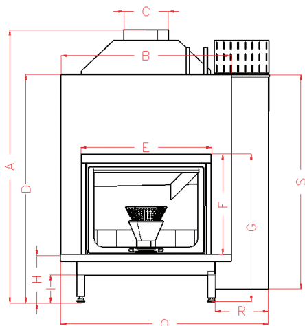
Frontale / Front view
