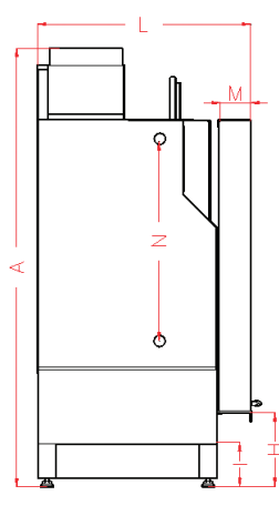
Laterale / Side view
